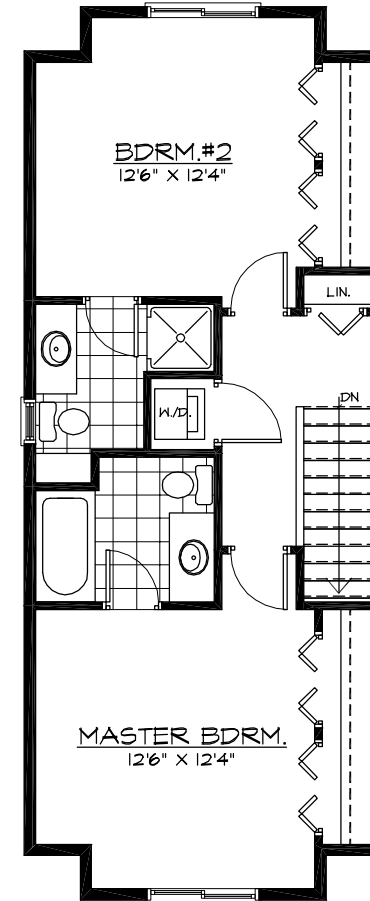
UPPER FLOOR 620 SQ. FT.
