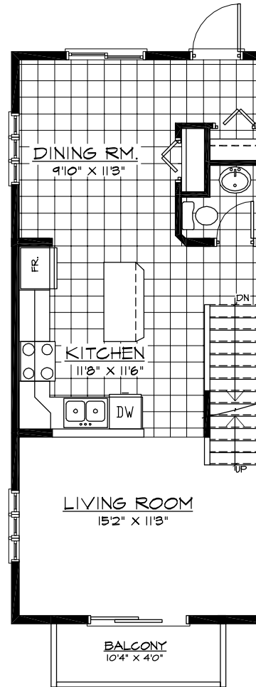
MAIN FLOOR 576 SQ. FT.
